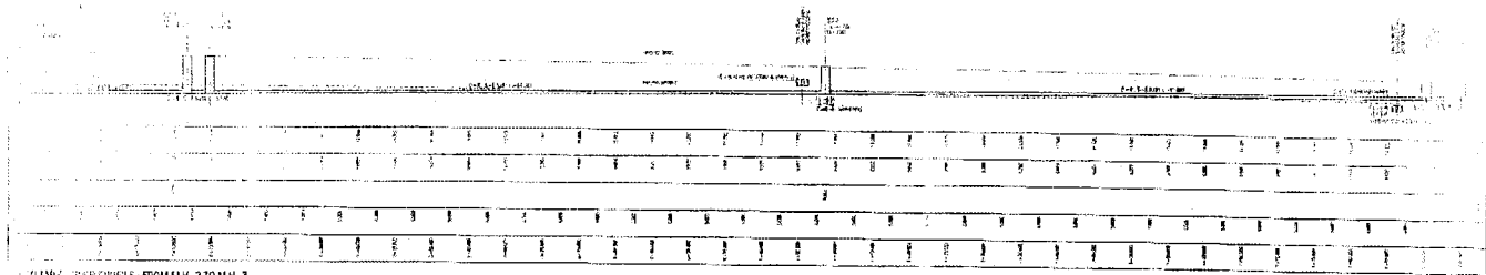
SANITARY SEWER PROFILE FROM M.H. -2 TO M.H. -1
