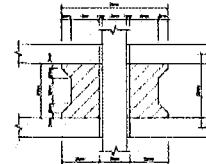
SPOOLS DETAIL
