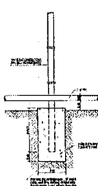
SECTION 12 NOT TO SCALE
