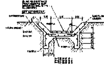
OUTFLOW DITCH
