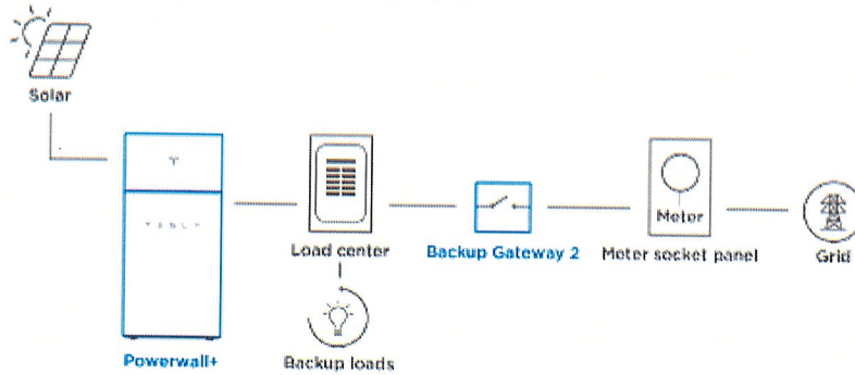
Powerwall+ with Backup Gateway 2 for Whole Home Backup
