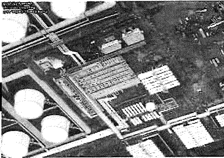
PUMA Energy Caribe Propane/ Butane Transfer Station, Bayamón, PR
