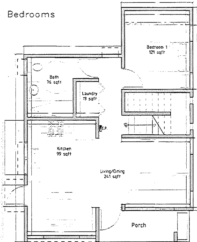
FIRST FLOOR PLAN Scale: 3/16" = 1'-0" Area: 758 sqft
