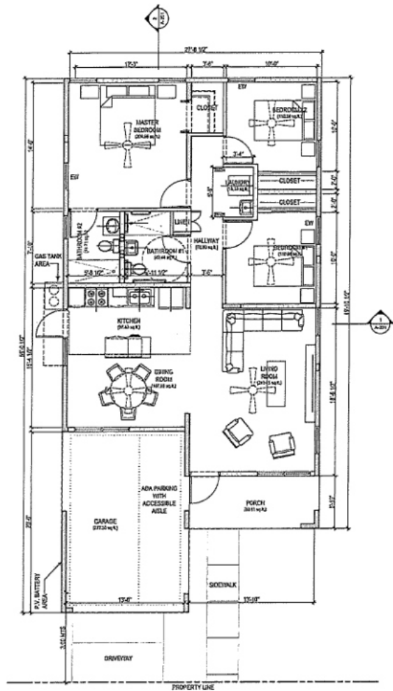
GROUND FLOOR PLAN SCALE: 1/4"
