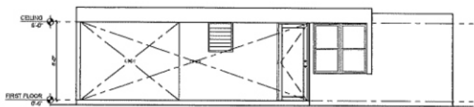
FRONT ELEVATION SCALE: 1/4"
