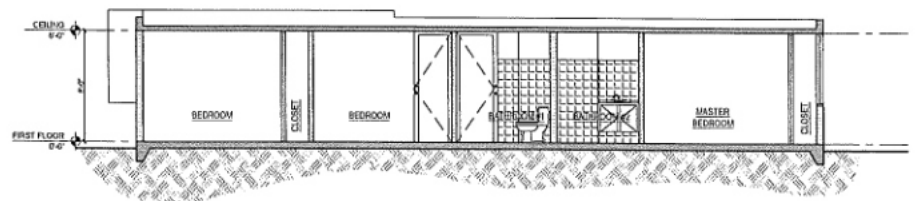
PROPOSED SECTION SCALE: 1/4"
