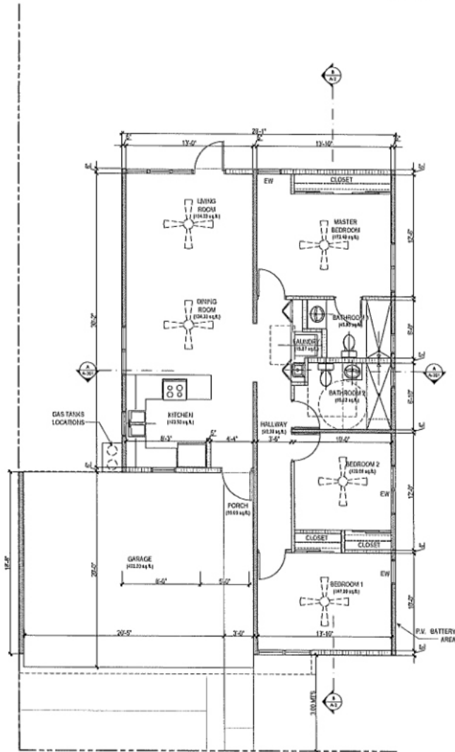
GROUND FLOOR PLAN SCALE: 1/4"
